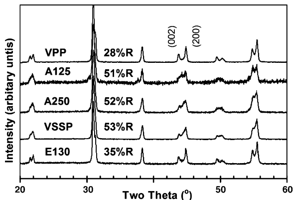
Fig. 3. XRD profiles for the five fibre types. Proportion of rhombohedral phase (%R) has been indicated for each material.
