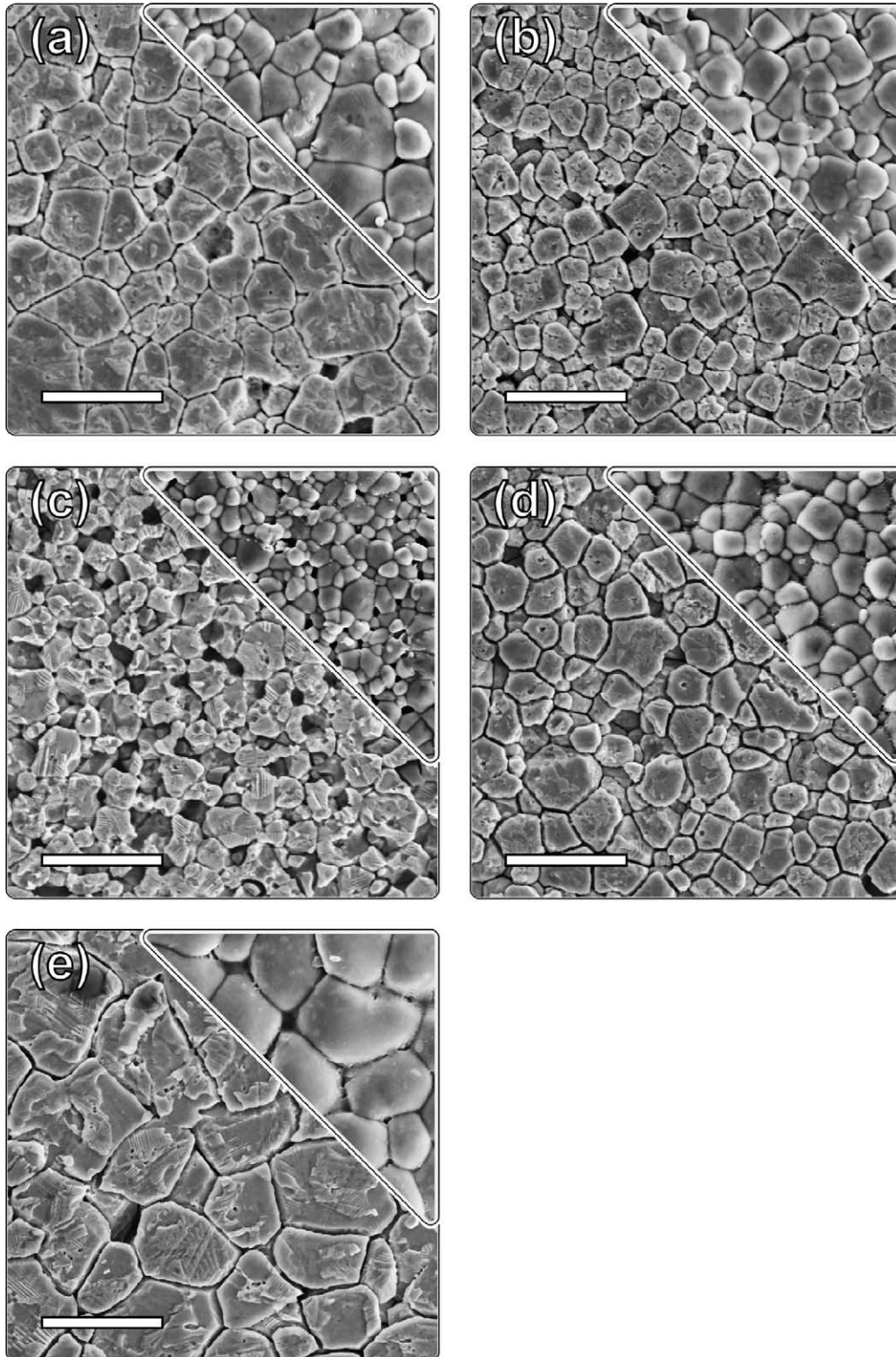
Fig. 2. Secondary electron images of polished fibre surfaces used to determine grain size, with inset (top right) of grains inspected along fibre exterior: (a) A125; (b) A250; (c) E130; (d) VPP and (e) VSSP. Scale bar: 10 \mu\text{m} .
