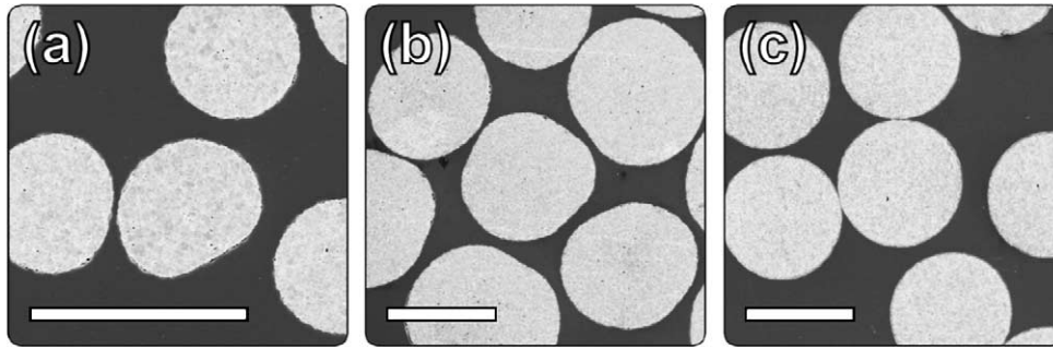
Fig. 1. Secondary electron images of fibre cross-sections: (a) A125; (b) VSSP and (c) VPP. Scale bar: 200 \mu\text{m} .
